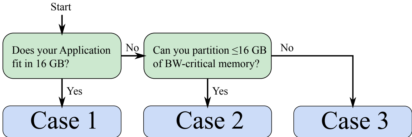
Figure 4: Flowchart for HBM usage.
